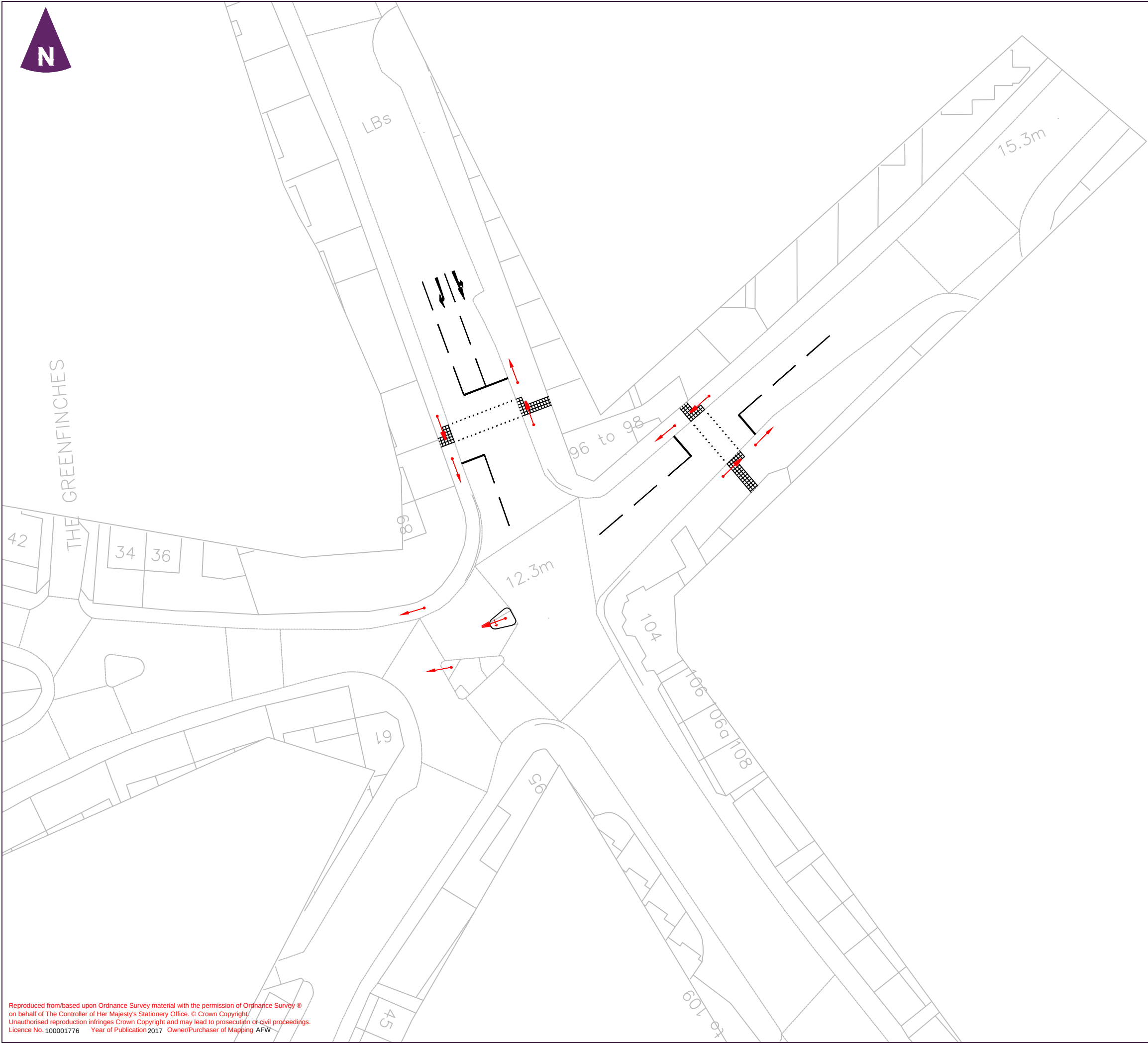
Figure 7.10 Jct 16 A254/B2052 Mitigation proposal
